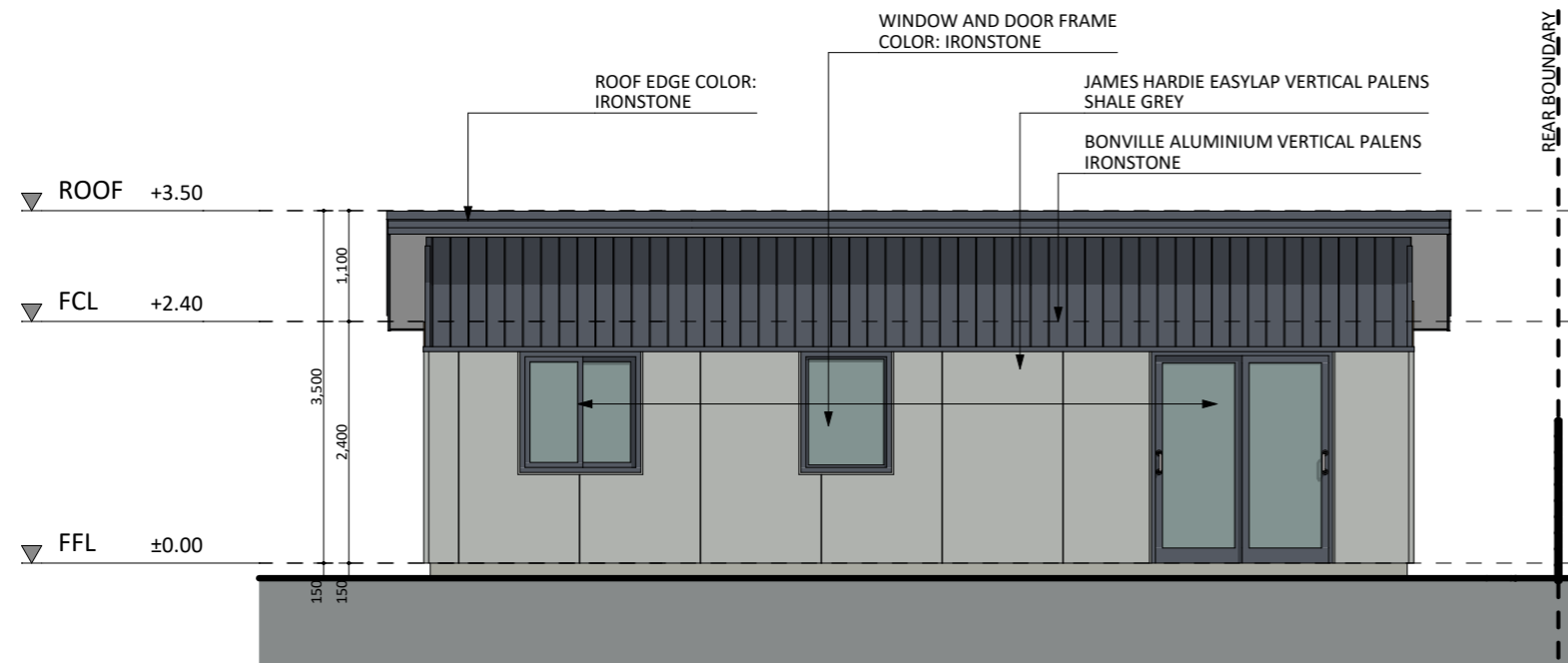
SOUTH ELEVATION
