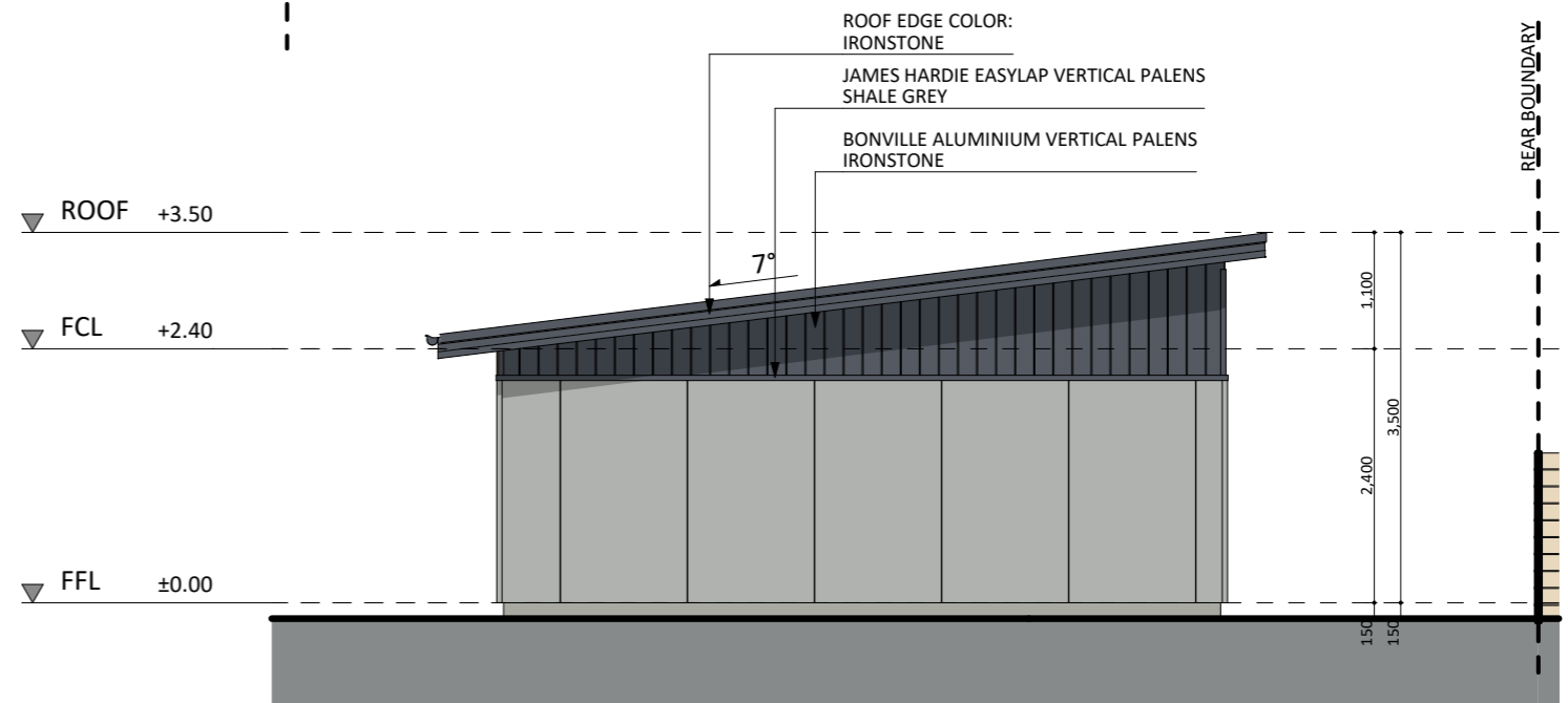
WEST ELEVATION
