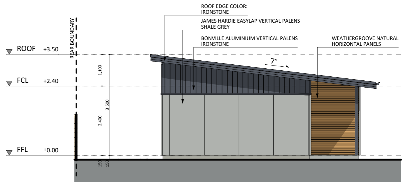
EAST ELEVATION
