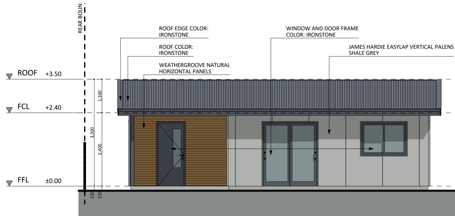
NORTH ELEVATION
