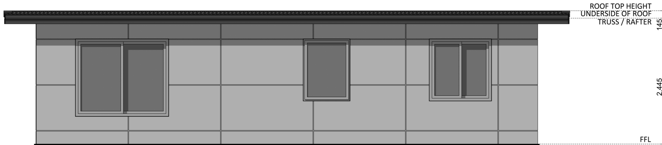
ELEVATION 03
