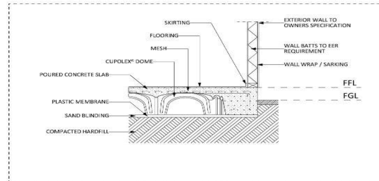
DETAIL 2 1:20
