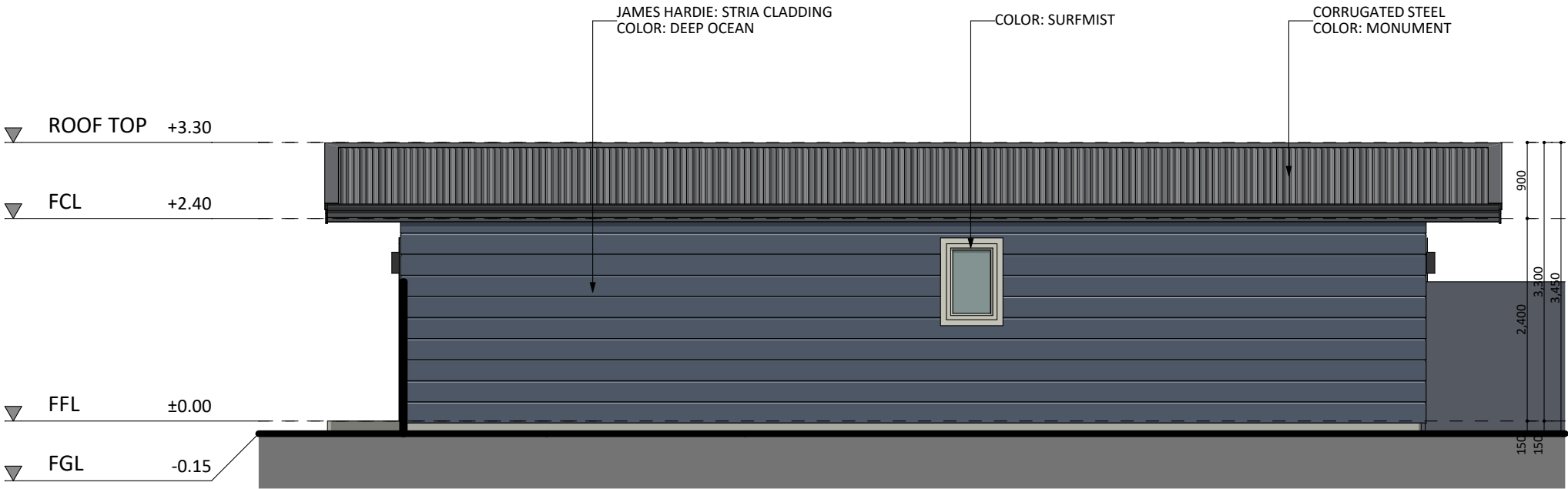
NORTH-EAST ELEVATION
