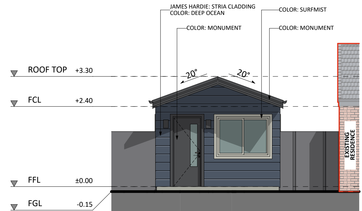
SOUTH-EAST ELEVATION
