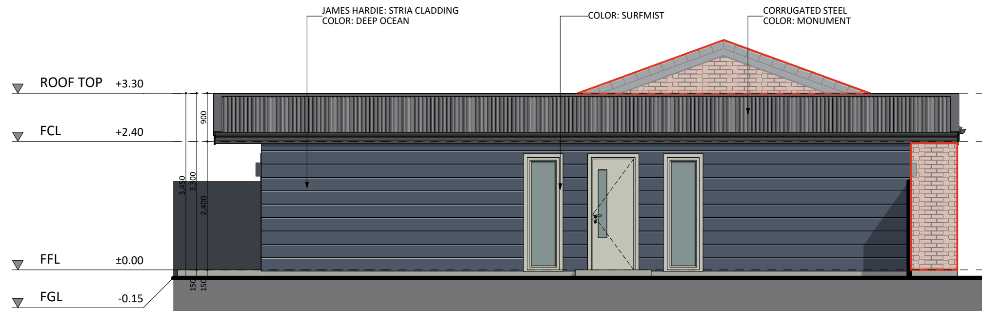
SOUTH-WEST ELEVATION
