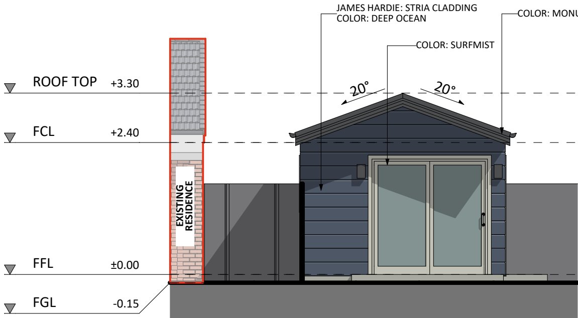
NORTH-WEST ELEVATION
