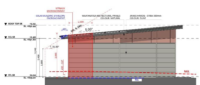
ELEVATION 03
