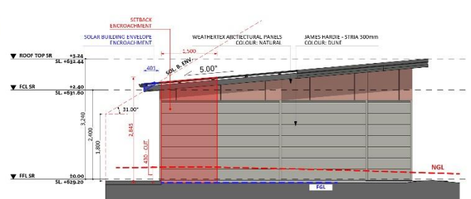
ELEVATION 03
