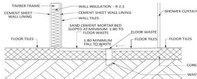
ADAPTABLE SHOWER RECESS SECTION SCALE 1:15
