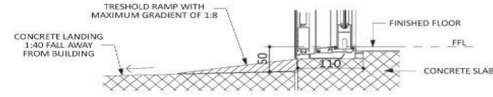
ACCESSIBLE ENTRY SECTION ALUMINIUM SLIDING DOORS SCALE 1:5
