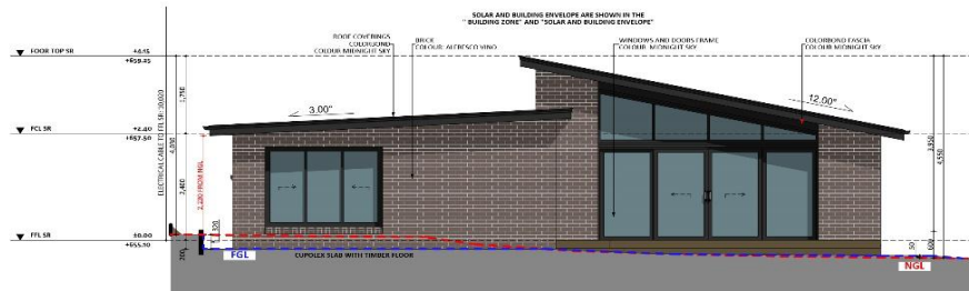
SOUTH-WEST ELEVATION
