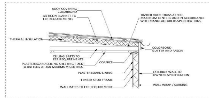
DETAIL 4 1:20
