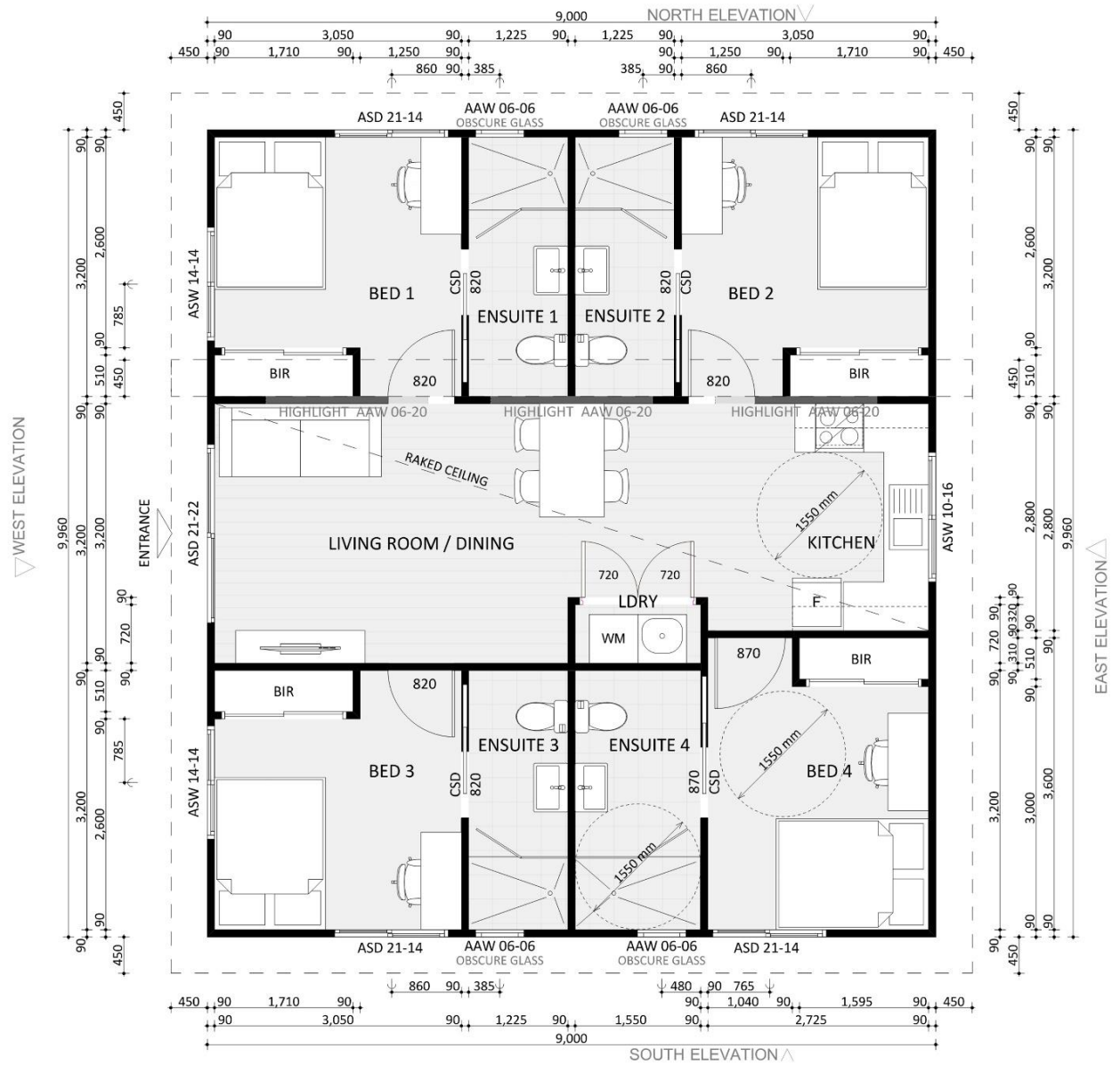
FLOORPLAN_DIMENSION_DESIGN_488
